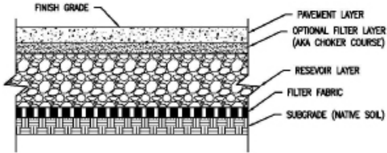
TYPICAL SECTION— PERVIOUS CONCRETE OR POROUS ASPHALT SCALE: NTS
