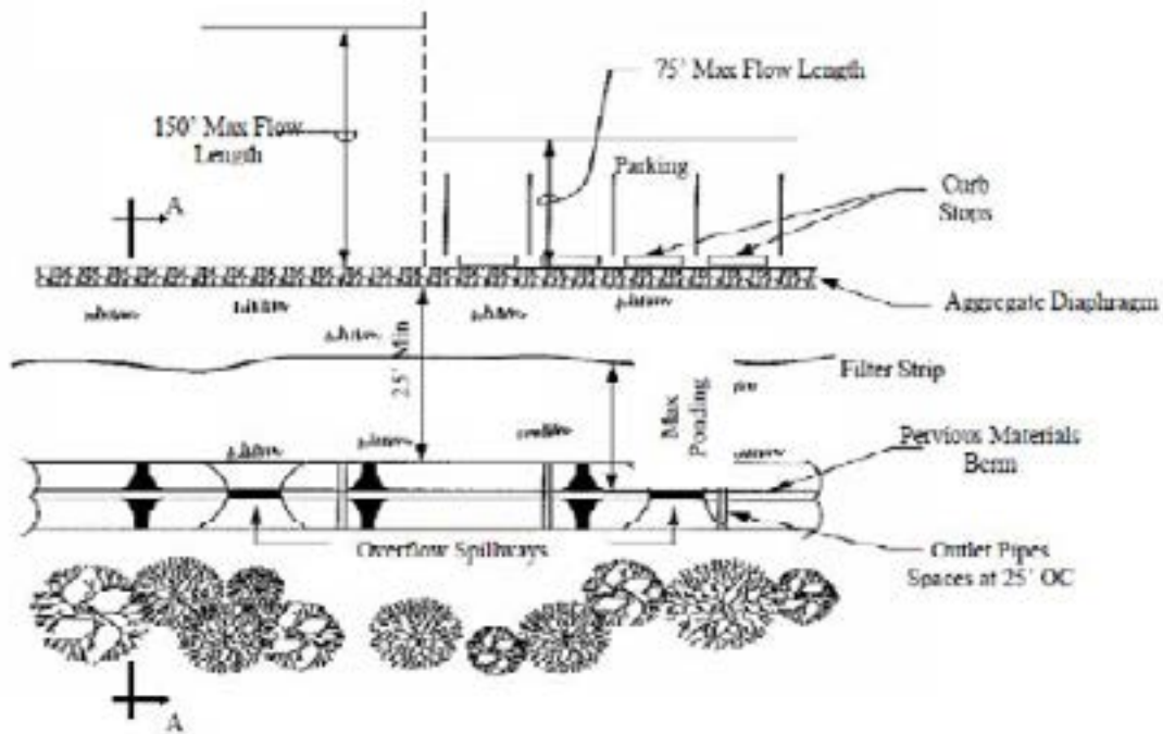
Detail "A" Plan View, Not to Scale
