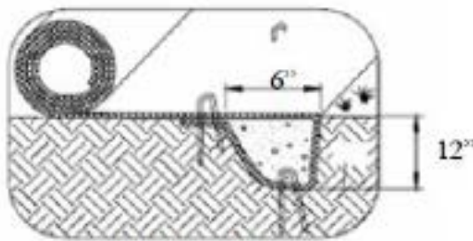
Initial Channel Anchor Trench Not to Scale See Note 3
