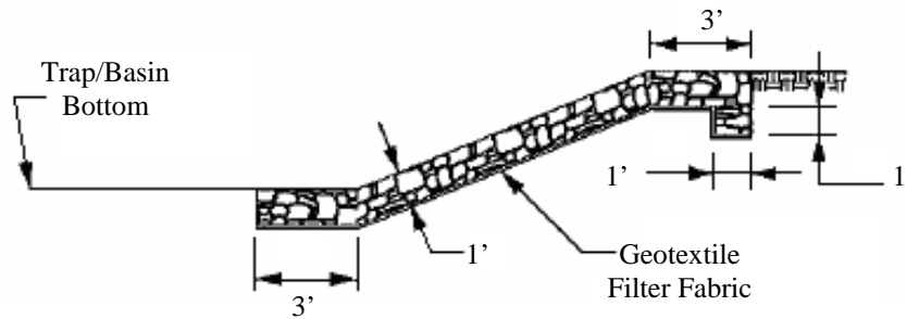
Centerline Profile View Not to Scale
