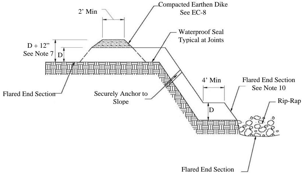
Section “A”
