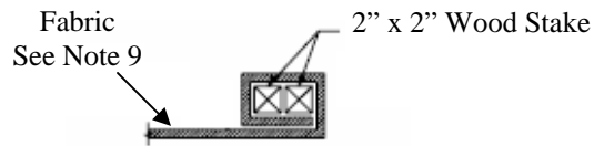
END STAKE DETAIL "D" (TOP VIEW)
