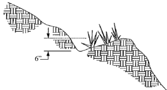
Furrow Detail "C" Not to Scale
