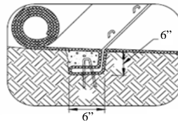
Intermittent Check Slot Not to Scale
