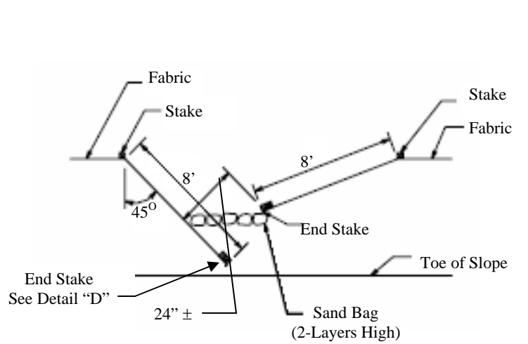
OPTIONAL MAINTENANCE OPENING DETAIL "C"
