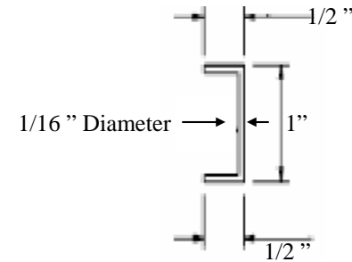
STAPLE DETAIL
