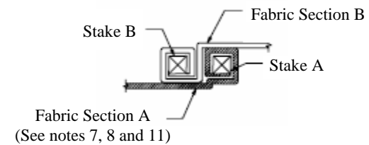
JOINING SECTION DETAIL "G" TOP VIEW
