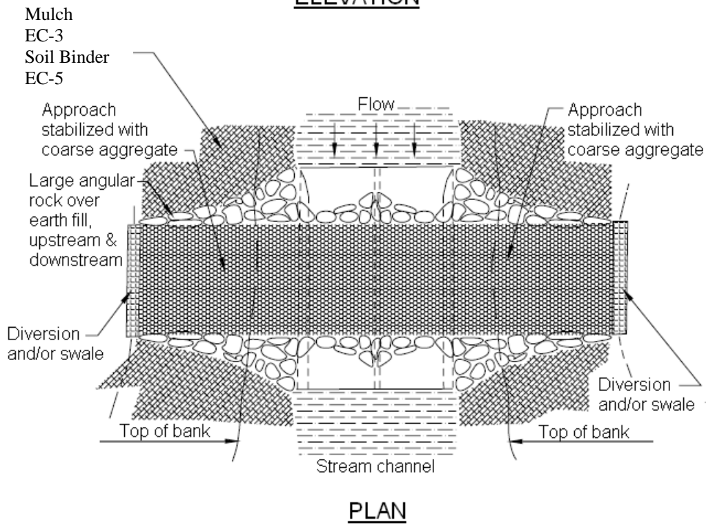
TYPICAL CULVERT CROSSING NOT TO SCALE
