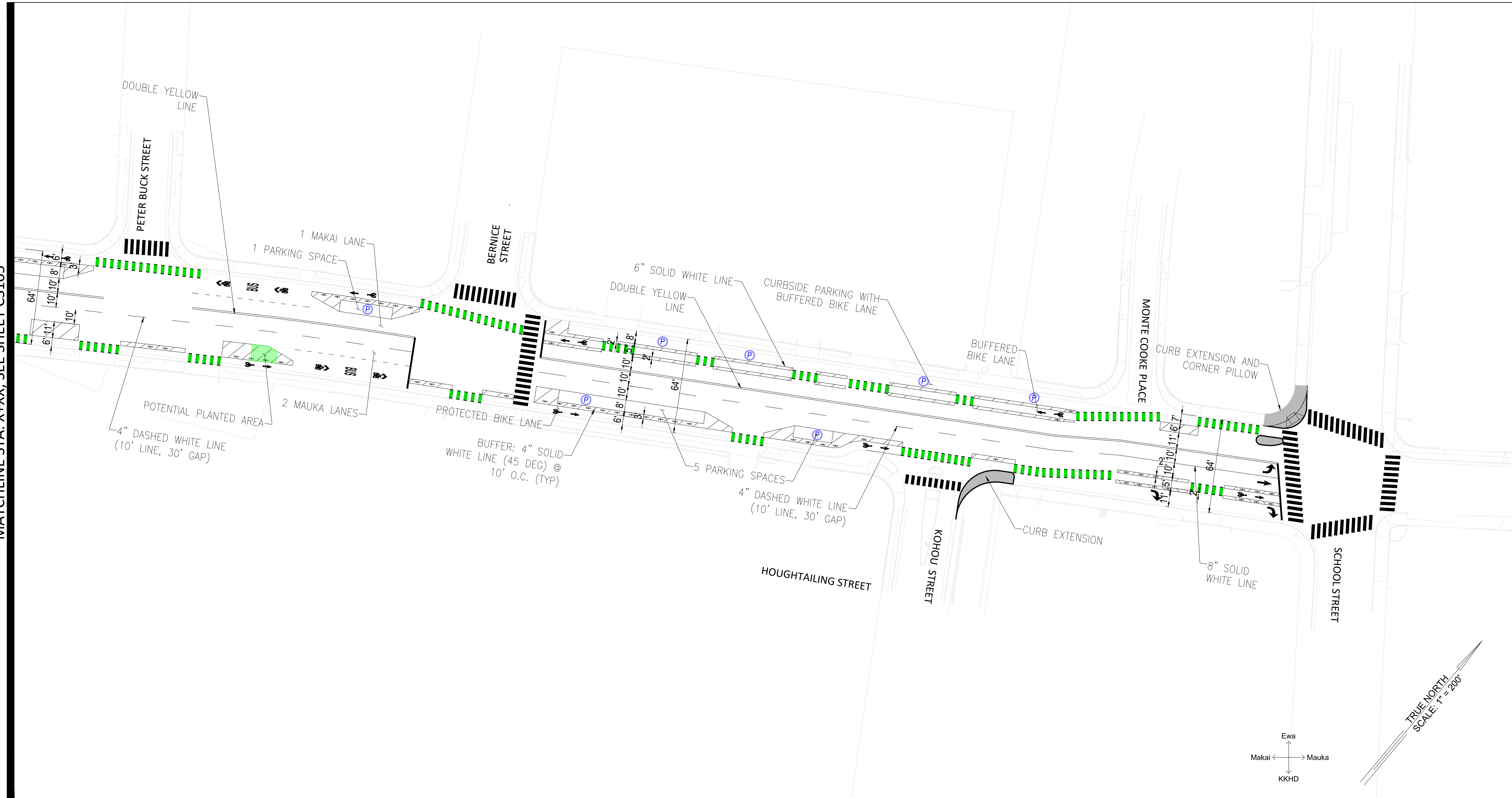
SITE AND STRIPING PLAN - HOUGHTAILING ST SCALE: 1" = 40'
